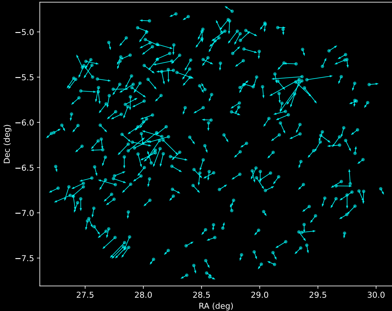
APOGEE DR17 Noise Stream Proper Motion Vectors (n=279)
