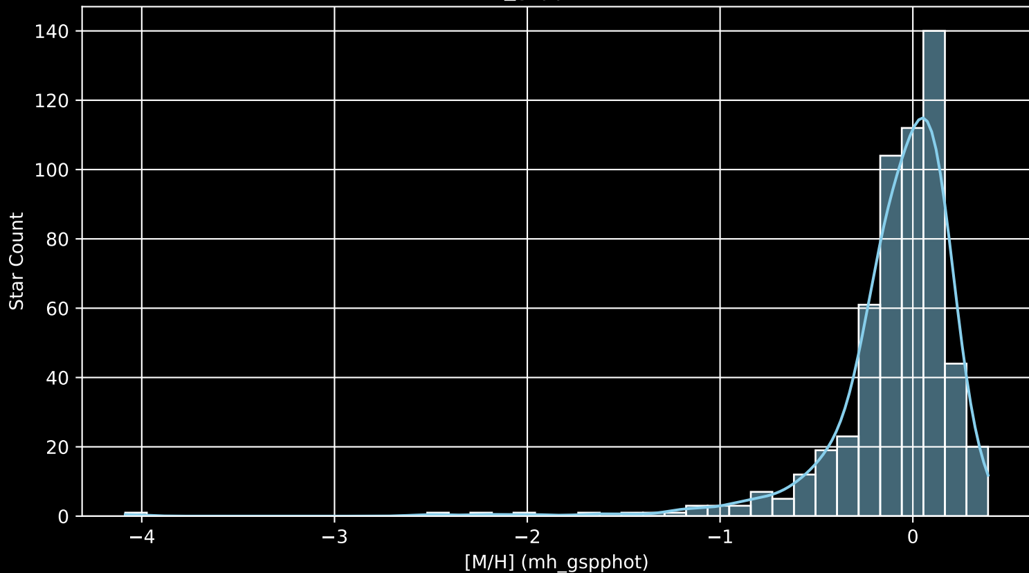
APOGEE DR17 Field: [030-08 [M/H] (mh_gspphot) (n= 564)
