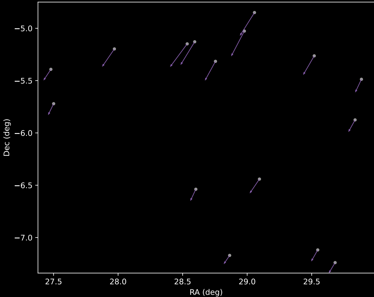
APOGEE DR17 Cluster 28 Proper Motion Vectors (n=16)
