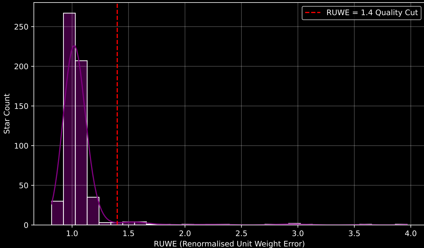
GAPOGEE DR17 Field [030-08] RUWE Distribution (n= 564)
