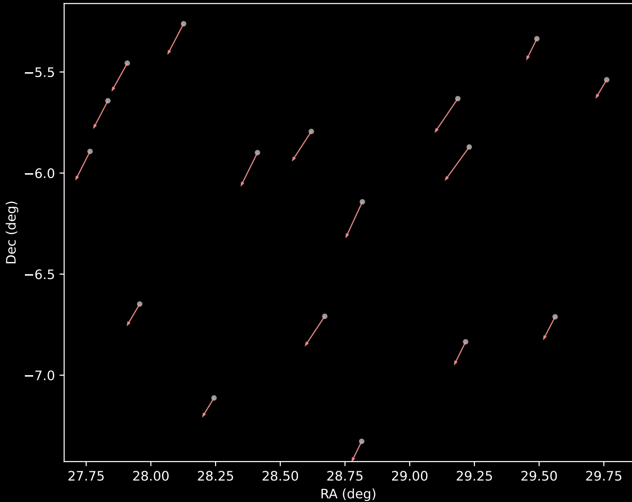
APOGEE DR17 Cluster 27 Proper Motion Vectors (n=17)
