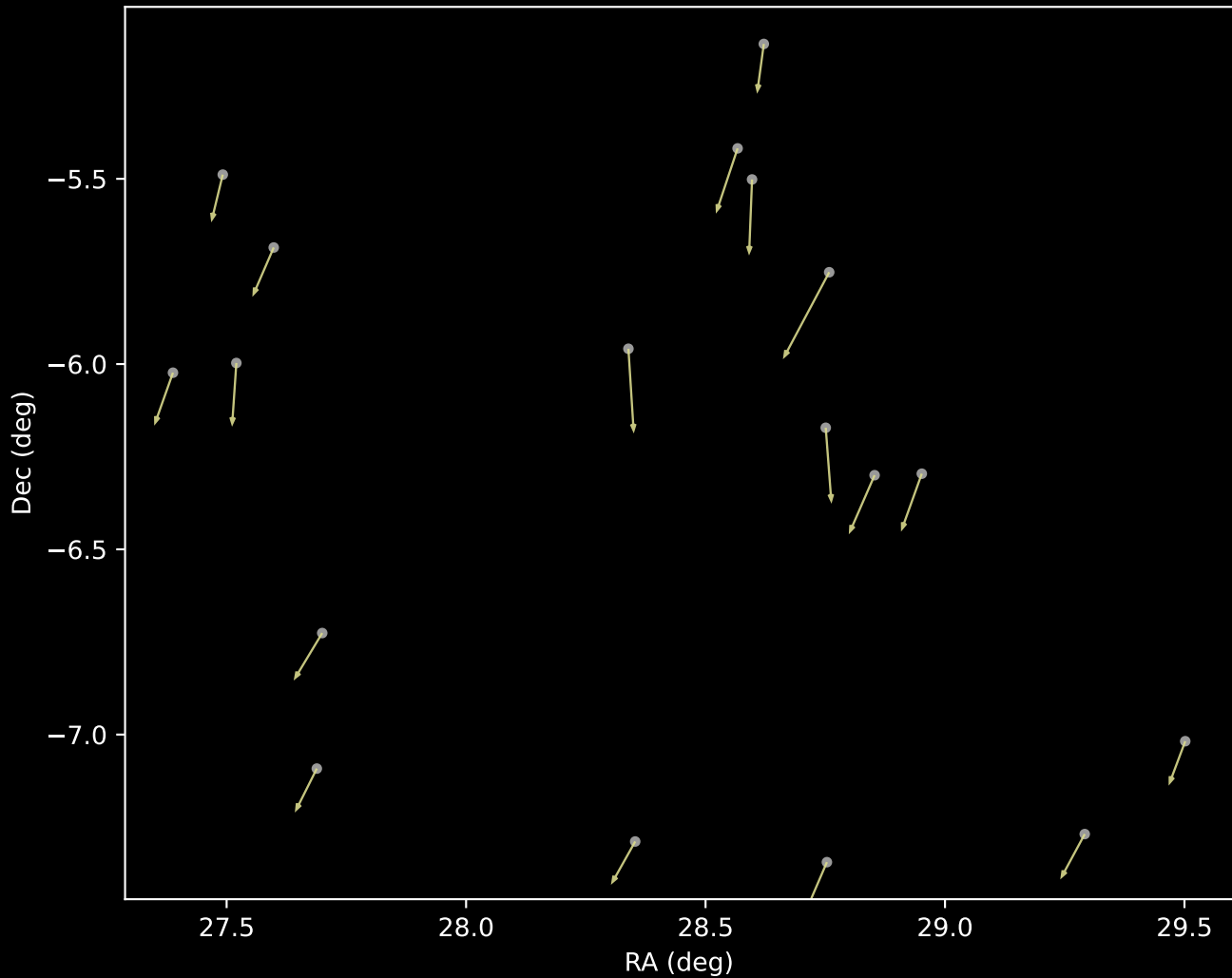
APOGEE DR17 Cluster 17 Proper Motion Vectors (n=18)
