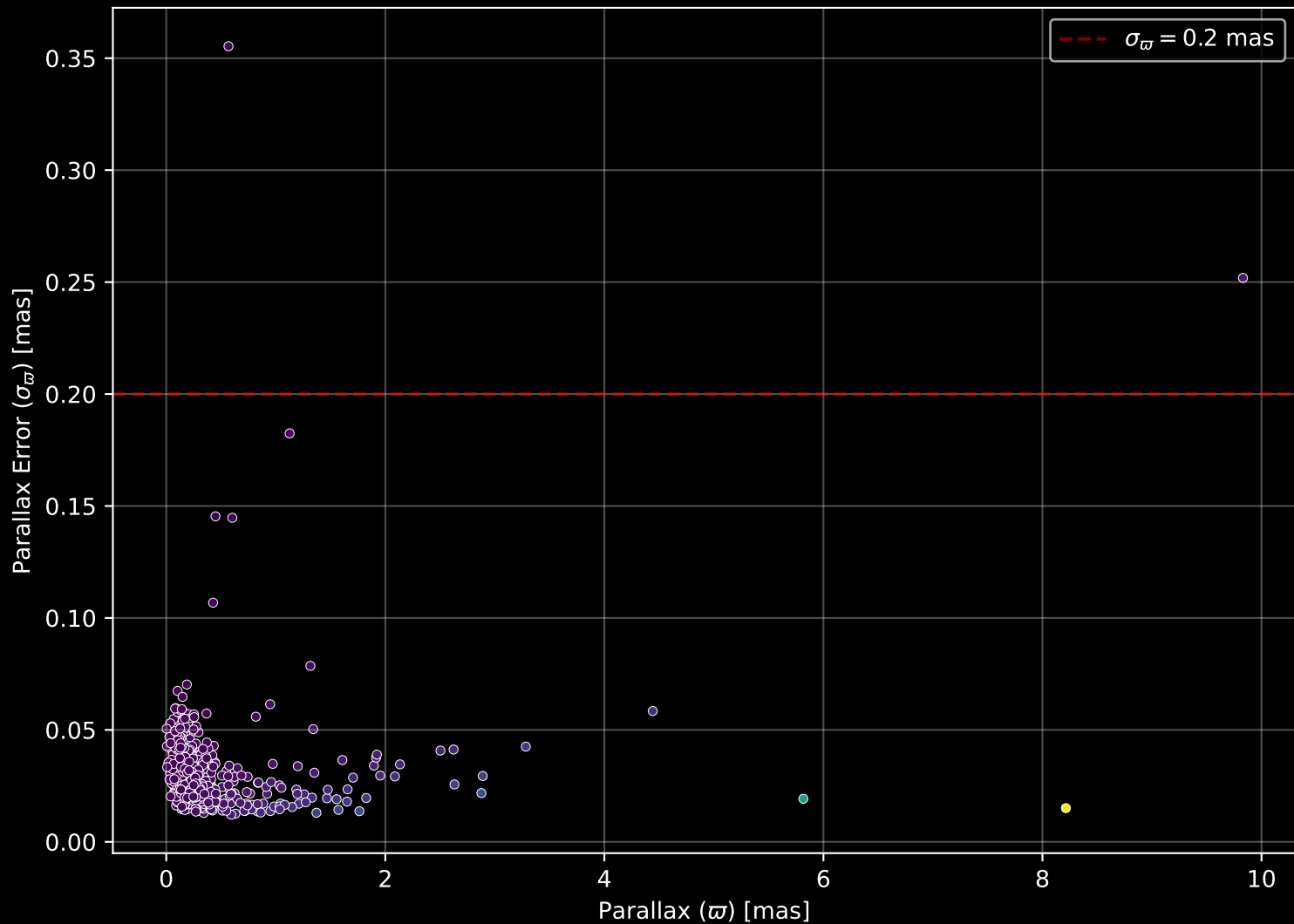
APOGEE DR17 Field: [030-08] Parallax Quality (n= 568)
