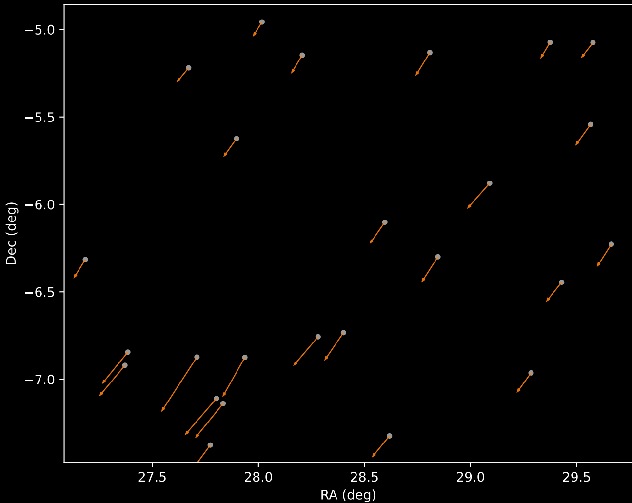
APOGEE DR17 Cluster 22 Proper Motion Vectors (n=25)
