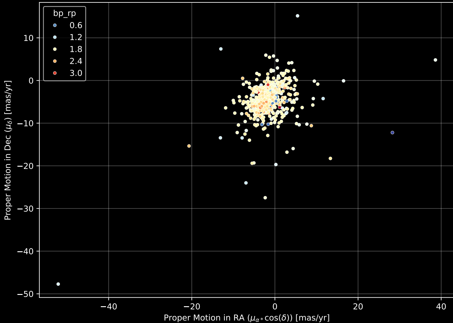
APOGEE DR17 Field: [030-08] Proper Motion Diagram (n= 568)
